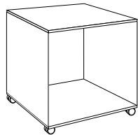
trolley 1 width × depth × height: 430 × 430 × 450 mm white or black
