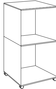
trolley 3 width × depth × height: 430 × 430 × 850 mm white or black
